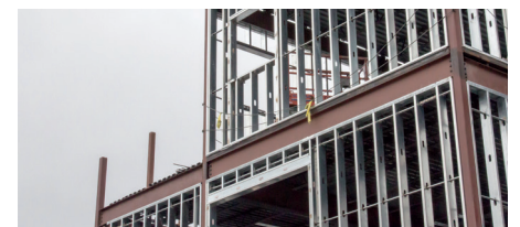
Fastening drywall track to steel
